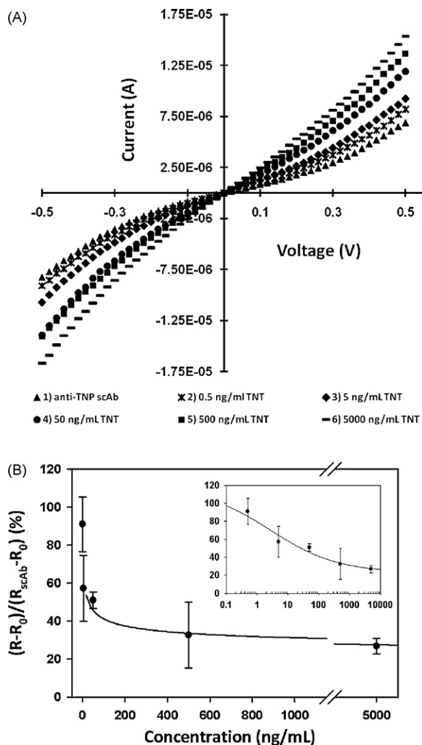
Fig. 3. Sensor response to different concentrations of TNT; (A) I - V plot according to the each concentration of TNT; anti-TNP scAb was bound to functionalized SWNTs (▲), 0.5 ng/mL (✕), 5 ng/mL (◆), 50 ng/mL (●), 500 ng/mL (■) and 5000 ng/mL (◼) of TNT were added. (B) Calibration curve of the sensor for TNT in buffer. Inset graph represents a function of the logarithm of concentration. Each data is an average of three measurements, and error bar stands for the standard deviation.
