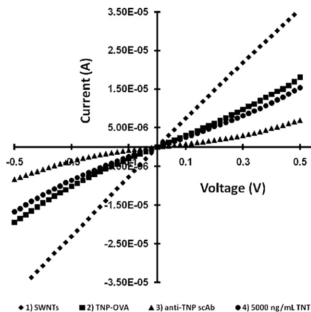
Fig. 2. Sequential responses of the sensor during the fabrication and the sensing. When TNP-OVA was immobilized on the SWNTs, the slope of the I - V plot decreased due to accumulation of negative charge of the protein. Antibody binding to TNP on the SWNTs also led to a decrease of the slope. After adding TNT, the slope was increased back; Bare SWNTs (◆), after modification with OVA-TNP (■), incubation with anti-TNP scAb (▲), and treatment with 5000 ng/mL of TNT (●).
