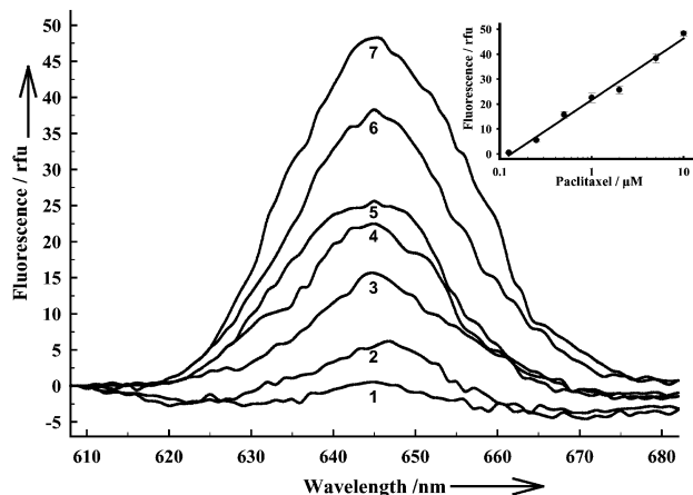
Fig. 3 Difference spectra of TCPP + tubulin + Taxol ® – TCPP plus tubulin. The Taxol ® concentration ranges from 0.125 \mu\text{M} (trace 1) to 10 \mu\text{M} (trace 7). Traces 2, 3, 4, 5 and 6 represent 0.25, 0.5, 1.0, 2.0 and 5.0 \mu\text{M} Taxol ® , respectively. The inset shows the linear relationship between the intensity of the peak at 645 nm and the Taxol ® concentration.
