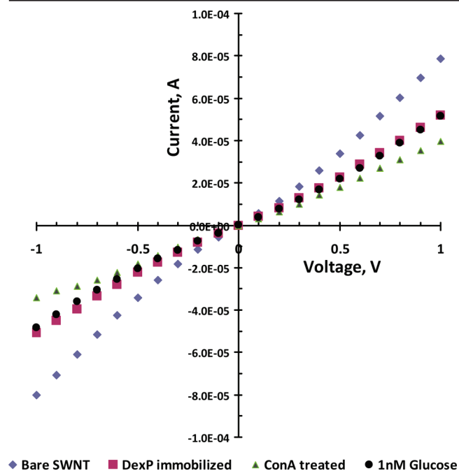
Figure 2. I – V characteristics of the biosensor at various stages of fabrication and upon addition of glucose.
